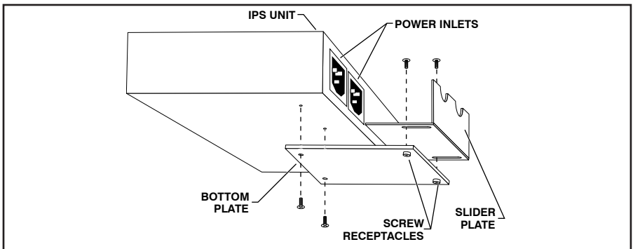
Figure 1: IPS Series Cable Keeper Installation (Slider Style Cable Keeper)
